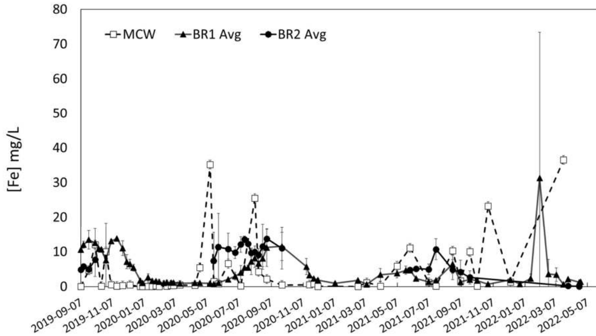
Figure 8. Iron in mg/L, of mine-contact water (MCW, empty square and dashed line), average BR1 (BR1 Avg, black triangle and full line) and average BR2 (BR2 Avg, black cycle and full line) function of time.
